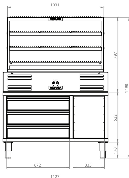
VISTA FRONTAL
