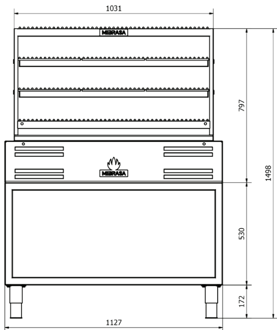
VISTA FRONTAL
