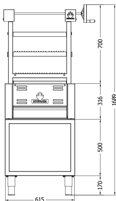
VISTA FRONTAL
