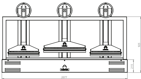
VISTA FRONTAL
