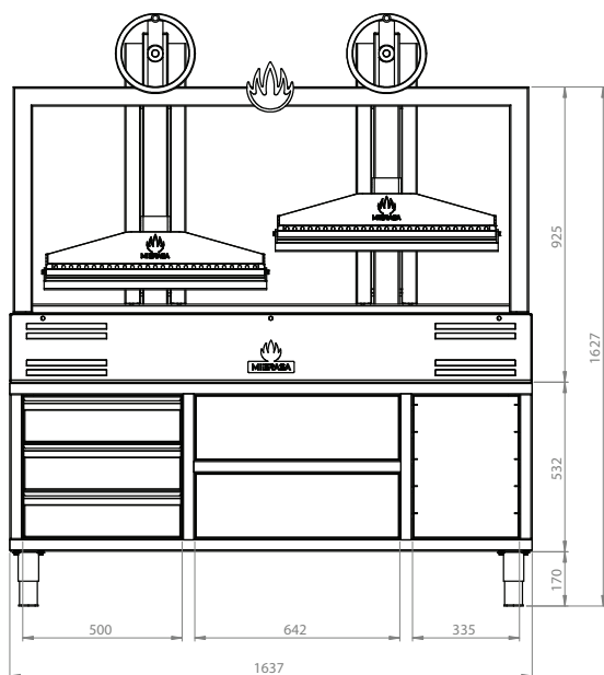
VISTA FRONTAL
