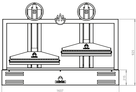
VISTA FRONTAL
