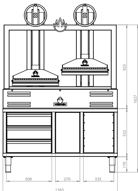
VISTA FRONTAL
